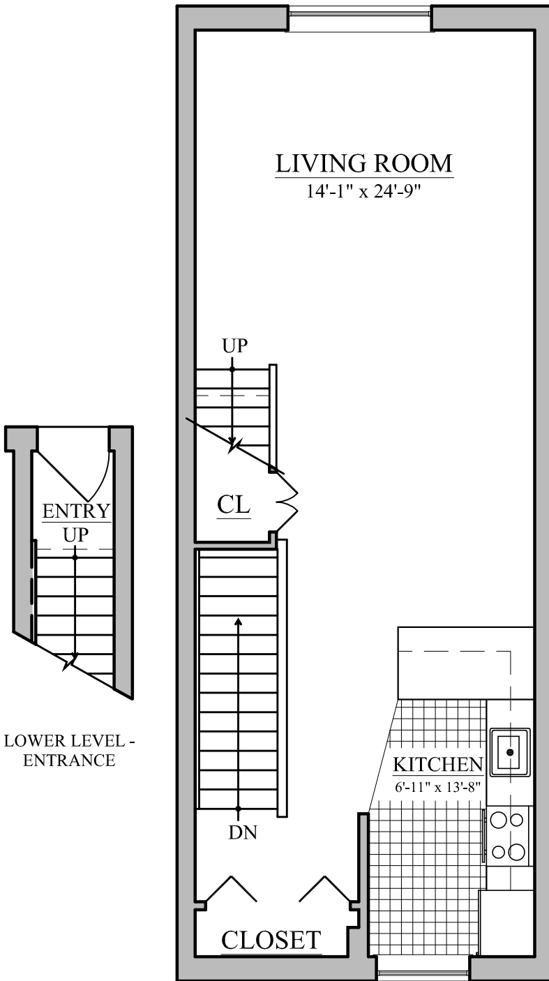
FIRST FLOOR
